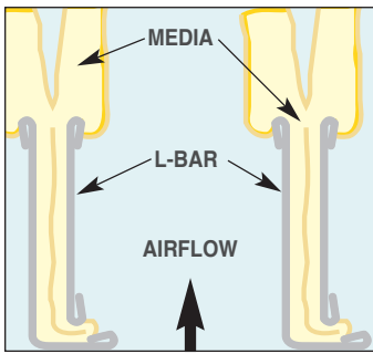
Interlocked Pocket Support Frames
