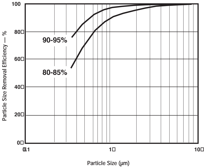
Composite Minimum Efficiency Curve
