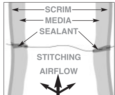
Interlocked Pocket Support Frames
