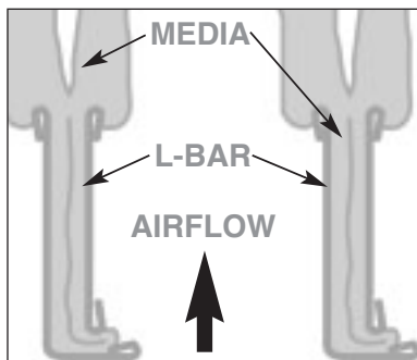
Leak-free Span Stitching
