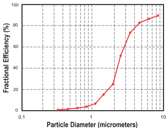
Initial Efficiency vs. Particle Diameter
